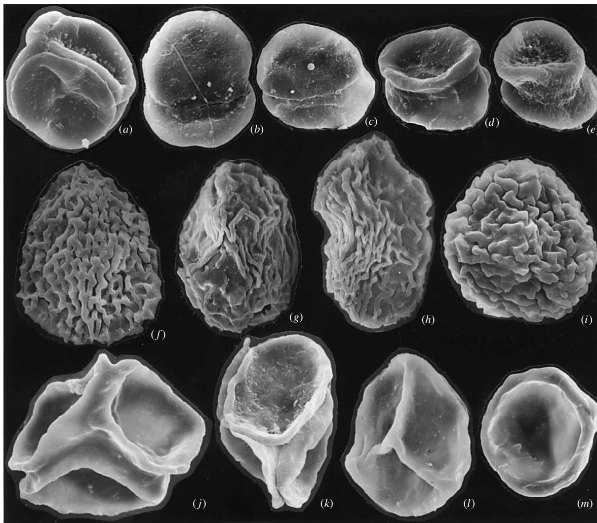
Figure 3. SEM images of dispersed early land plant spores. ( a–i ) From the type area for the Caradoc, Shropshire, England Caradoc, Late Ordovician (Wellman 1996); ( j–m ) from the Silurian inliers along the southern margin of the Midland Valley of Scotland (early Wenlock, Late Silurian) (Wellman & Richardson 1993). ( a ) Naked, unfused, permanent tetrad ( \times 2000 ); ( b,c ) naked, unfused, permanent dyad ( \times 1500 ); ( d,e ) naked, fused, permanent dyad ( \times 1500 ); ( f–h ) envelope-enclosed permanent dyad ( \times 1500 ); ( i ) envelope-enclosed permanent monad ( \times 1500 ); ( j ) naked, fused, permanent tetrad ( \times 1210 ); ( k ) loose tetrad ( \times 1070 ); ( l ) laevigate trilete spore ( \times 1380 ); ( m ) laevigate hilate monad ( \times 1230 ).
